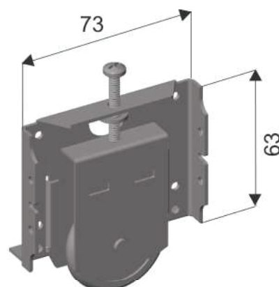
Section No.DR140 Adjustable Wardrobe Carriage Material: Zinc Seal Standard Roller: DR35 Max Load: 25kg
