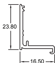
Section No. 34732 Hook Bead 16.5x23.8mm 0.154kg/m, per 90.09
