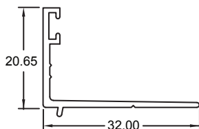
Section No. RB-981 Double Glazing Bead 32x20.65mm 0.198kg/m, per 121
