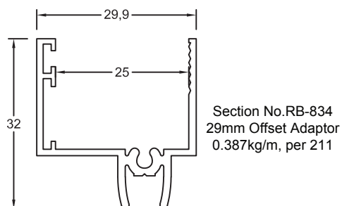
Offset Adaptor
