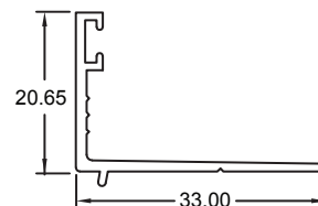
Section No. RB-894 Double Glazing Bead 33x20.65mm 0.198kg/m, per 121
