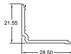
Section No. 34736 Bead 28.5mm 0.194kg/m, per 100
