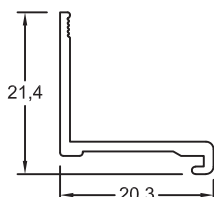
*Section No. RB-893 20.3mm Hook Bead 0.153kg/m, per 86
