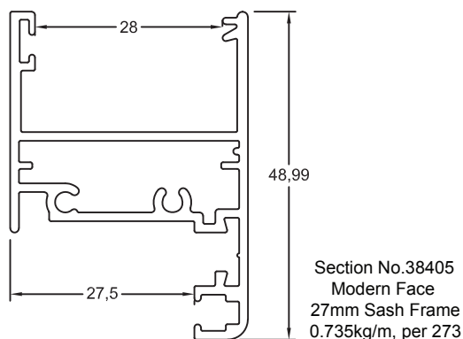
27mm Sash
