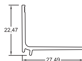
Section No. RB-264 Universal Bead 0.175kg/m, per 101
