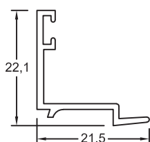
Section No. RB-246 New Stepped Bead 0.158kg/m, per 102
