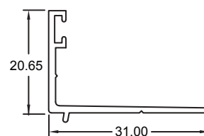
Section No. RB-980 Double Glazing Bead 31x20.65mm 0.194kg/m, per 120
