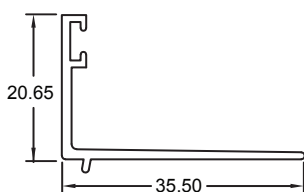
Section No. RB-978 Double Glazing Bead 35.5x20.65mm 0.209kg/m, per 127
