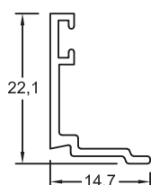
Section No. RB-247 Homestead Stepped Bead 0.136kg/m, per 85
