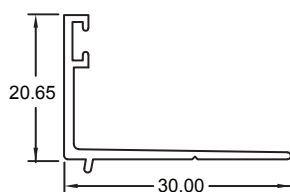
Section No. RB-979 Double Glazing Bead 30x20.65mm 0.19kg/m, per 117
