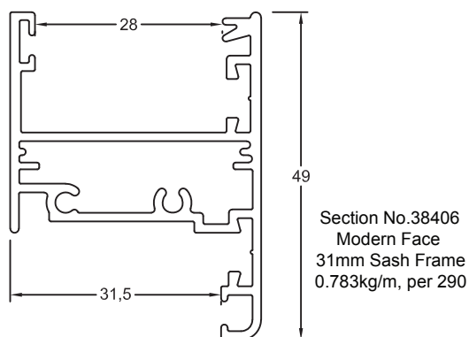
31mm Sash
