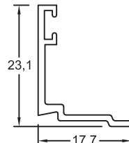
Section No. RB-248 Villa Stepped Bead 0.150kg/m, per 93
