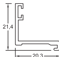
*Section No. RB-235 20.3mm Vantage Hook Bead 0.173kg/m, per 100
