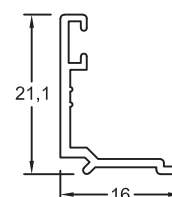
*Section No. RB-895 Vista Bead 0.131kg/m, per 88
