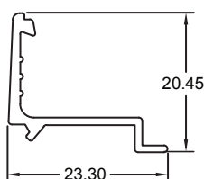
Section No. 36116 Stepped Bead 23.3x20.45mm 0.163kg/m, per 93.21
