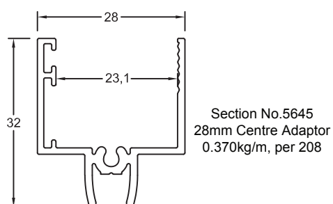
Centre Adaptor
