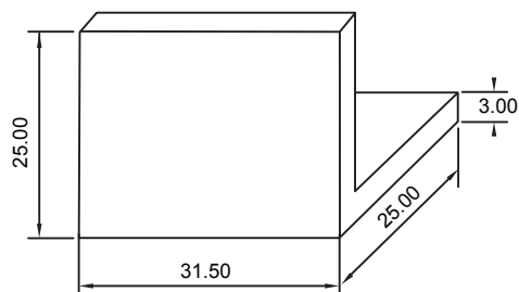
Section No. Cleat Retrofit 31.5mm Retrofit corner Cleat fit 34261 / 34262 / 38405 / 38406
