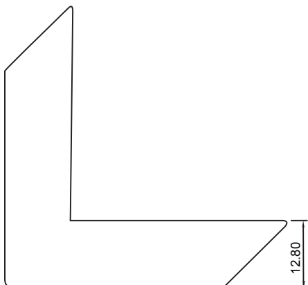
Section No.K024S Adaptor Gusset 12.80mm for Adaptor RB-233 / RB-237 / RB-834 / 5645
