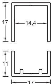
Section No.31018 Deep Bottom Channel 0.139kg/m, per 81
