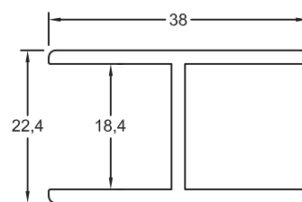
Section No. 30503 Radius H-Corner Jointer 0.509kg/m, per 191
