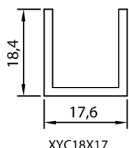
XYC18X17
