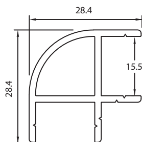
Section No. RB-984 15.5mm ID Corner Jointer, 17mm Rad 0.388kg/m, per 143.97
