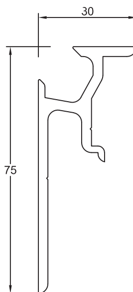
Section No. RB-190 1.018 kg/m, per 265
