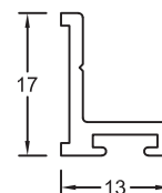
Section No. 6136 Door Stop 0.150kg/m, per 72
