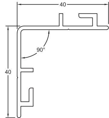
Section No.RB-374 40mm DRI Dual Angle 0.501kg/m, per 224
