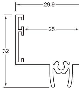
Section No.RB-834 29mm Offset Adaptor 0.387kg/m, per 211
