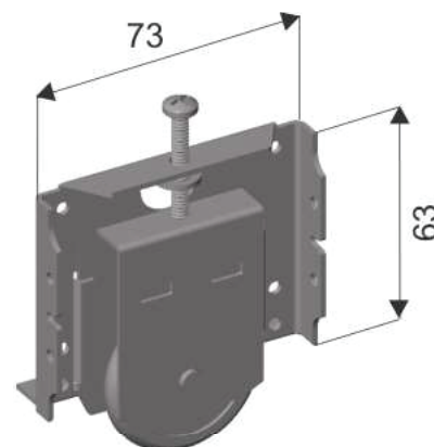
Section No.DR140 Adjustble Wardrobe Carriage Material: Zinc Seal Standard Roller: DR35 Max Load: 25kg
