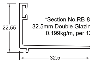
Section No.RB-265 35.5mm Double Glazing Bead 0.212kg/m, per 128
