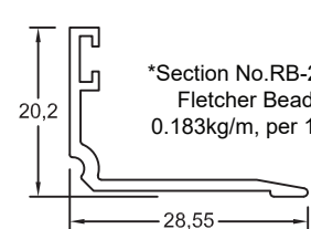
*Section No.RB-894 32.5mm Double Glazing Bead 0.199kg/m, per 121
