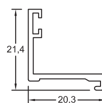
*Section No.RB-235 20.3mm Vantage Hook Bead 0.173kg/m, per 100
