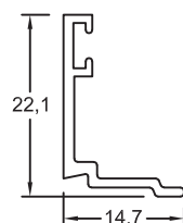
Section No.RB-247 Homestead Stepped Bead 0.136kg/m, per 85
