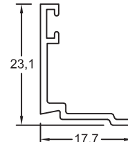
Section No.RB-248 Villa Stepped Bead 0.150kg/m, per 93
