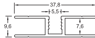
Section No. 6488 Jointer with Groove 0.260kg/m, per 172
