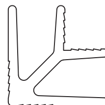
Section No.6868K Corner Stake For Z785
