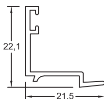
Section No.RB-246 New Stepped Bead 0.158kg/m, per 102
