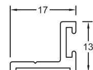
Section No.6136 Door Stop 0.150kg/m, per 72
