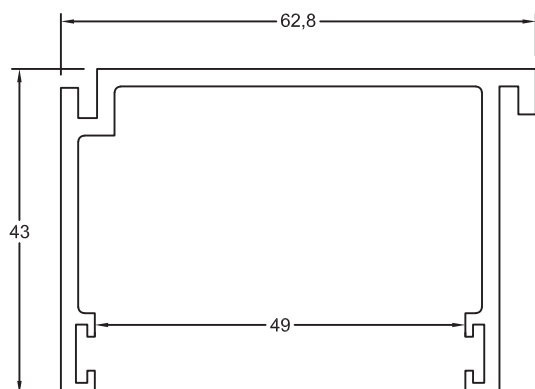
Section No. 5584 Head Track 0.987kg/m, per 340
