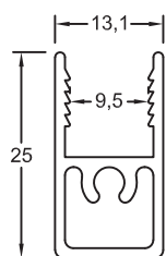
Section No.Z439 11mm Rail Frame 0.285kg/m, per 160
