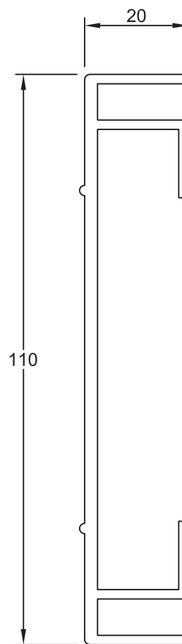
Section No.F4638 1.221 kg/m, per 418
