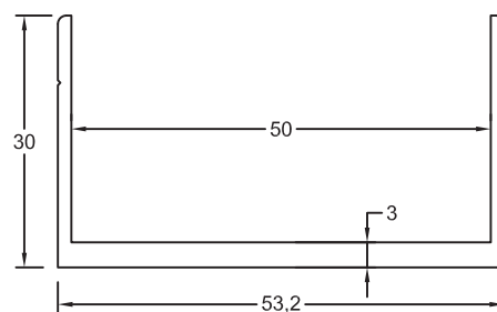
Section No.RB-472 50mm Heavy Channel 0.670kg/m, per 220
