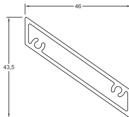
Section No. RB-452 Parallelogram Louvre 0.594kg/m, per 135
