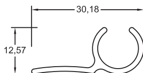
Section No. YLJ02552 11mm Awning 0.193kg/m, per 102
