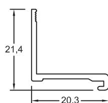
*Section No.RB-893 20.3mm Hook Bead 0.153kg/m, per 86
