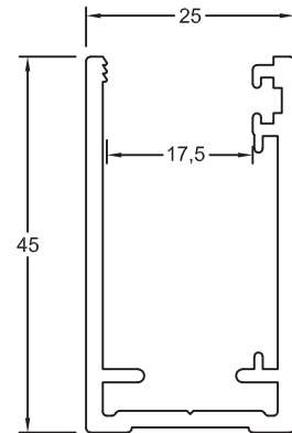
Section No.31427 Glazing Channel 0.693kg/m, per 271
