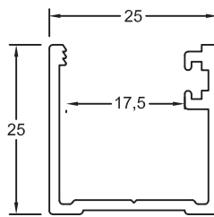
Section No.E770 Glazing Channel 0.387kg/m, per 167
