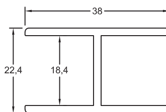
Section No.30503 Radius H-Corner Jointer 0.509kg/m, per 191
