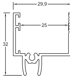
Section No.RB-237 29mm Offset Adaptor 0.376kg/m, per 216
