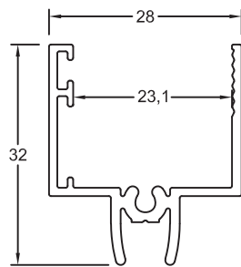
Section No.5645 28mm Centre Adaptor 0.370kg/m, per 208
