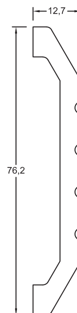
Section No.0732 75mm Threshold 1.154kg/m, per 181
