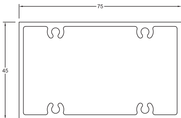
Section No.7771 Screw Port Box 1.532kg/m, per 240
