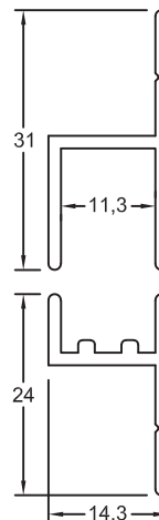
Section No.J031 Bottom Channel with Leg 0.191kg/m, per 94
