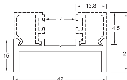
Section No. 5620 Vision Rail Infil 0.484kg/m, per 157
