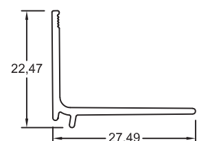
Section No.RB-264 Universal Bead 0.175kg/m, per 101
