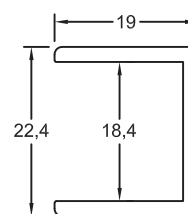
Section No.30504 Radius Cap 0.303kg/m, per 115
