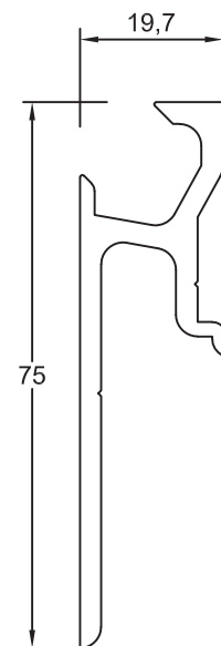
Section No. RB-087 0.941 kg/m, per 237
