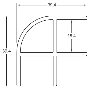
Section No.30505 Radius Corner Jointer 0.764kg/m, per 281
