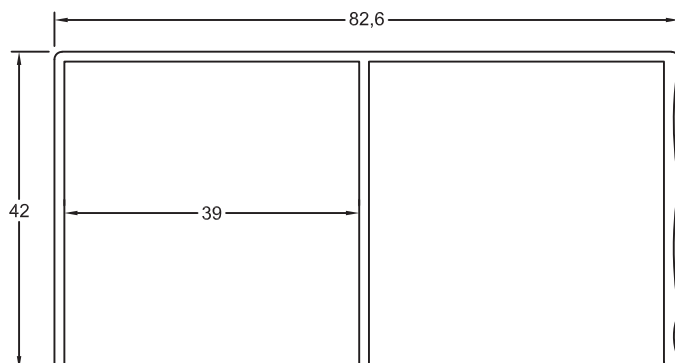
Section No.N924 82mm Double Head Top Guide 0.745kg/m, per 410
