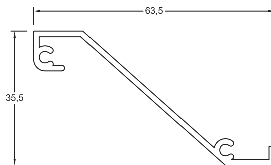
Section No. G452 63.5mm Louvre 0.438kg/m, per 211
