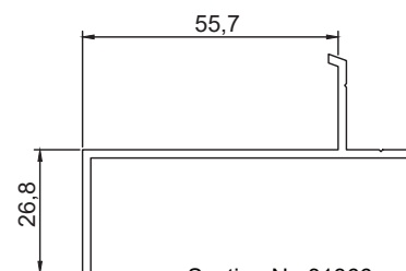
Section No.31366 0.582 kg/m, per 242
