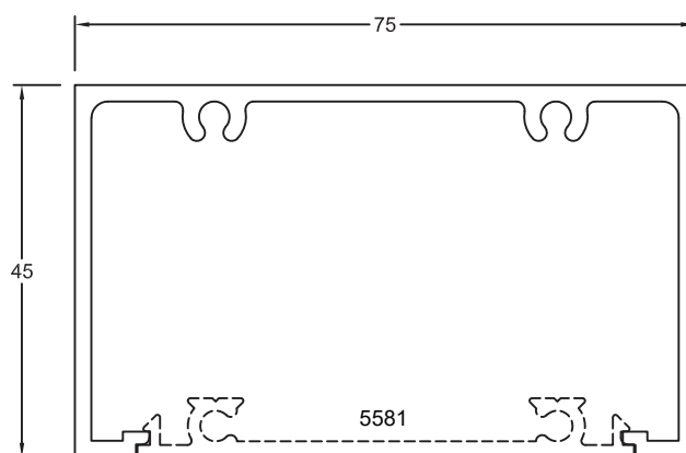
Section No.6726 Screw Port Channel 1.079kg/m, per 388
