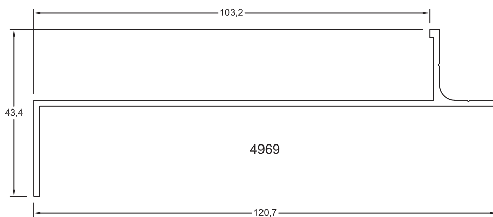
Section No. 4969 Sill Tray 0.703kg/m, per 329
