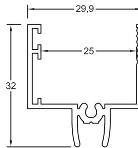
Section No.RB-233 29mm Centre Adaptor 0.376kg/m, per 216
