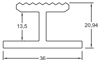
Section No. YLJ07668 13mm Walkway Mesh H Jointer 0.673kg/m, per 155
