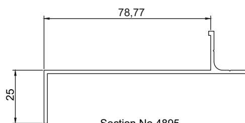
Section No.4895 0.595 kg/m, per 278
