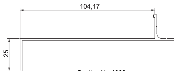
Section No.4969 0.703 kg/m, per 329
