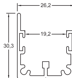
Section No.30973 26mm Sliding Door Track 0.421kg/m, per 210
