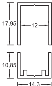
Section No.X076 Bottom Channel 0.119kg/m, per 79
