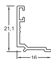
*Section No.RB-895 Vista Bead 0.131kg/m, per 88
