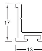
Section No. 6136 Door Stop 0.150kg/m, per 72
