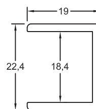
Section No. 30504 Radius Cap 0.303kg/m, per 115
