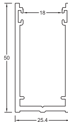
Section No.33604 Glazing Channel 0.742kg/m, per 276
