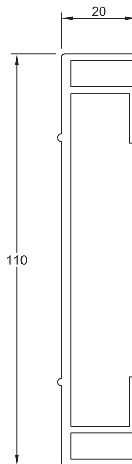
Section No.F4638 1.221 kg/m, per 418
