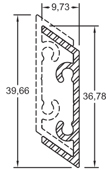
Section No. 5947 French Cleat 0.269kg/m, per 135
