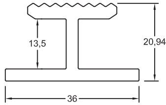
Section No. YLJ07668 13mm Walkway Mesh H Jointer 0.673kg/m, per 155
