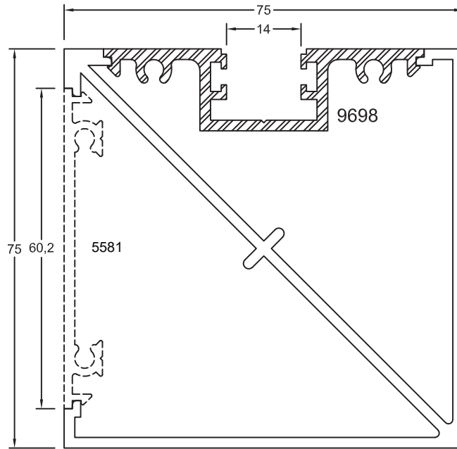
Section No.9698 Shallow Pocket Infil 0.429kg/m, per 182
