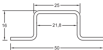
Section No. 0582 0.324kg/m, per 153
