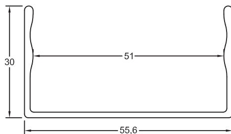
Section No. RB-043 51mm Channel 0.504kg/m, per 227
