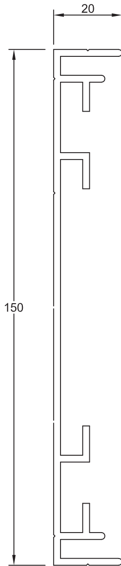
Section No.X540 1.418 kg/m, per 529
