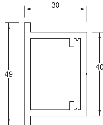
Section No.RB-830 1.170 kg/m, per 158
