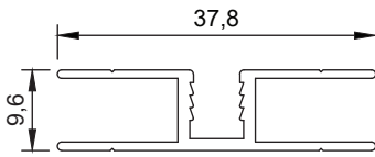
Section No. 6488 0.260 kg/m, per 172
