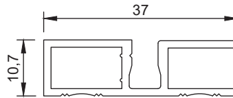
Section No. RB-122 0.355 kg/m, per 144
