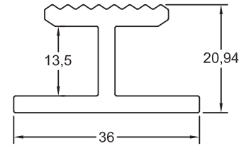
Section No.YLJ07668 0.673 kg/m, per 155
