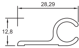
Section No.6595 0.237 kg/m, per 96
