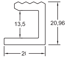
Section No.YLJ07669 0.445 kg/m, per 104
