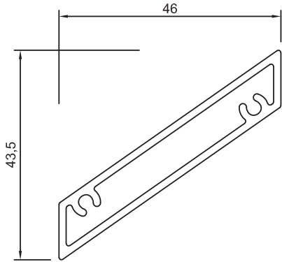
Section No.RB-452 0.594 kg/m, per 135
