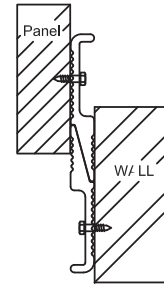
Instruction Drawing For RB-706
