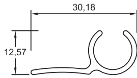
Section No.YLJ02552 0.193 kg/m, per 102
