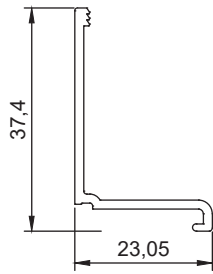
Section No. G674 0.247 kg/m, per 124.1
