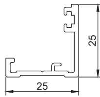
Section No. E772 0.284 kg/m, per 140.1
