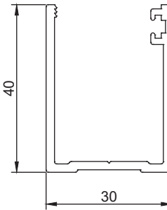
Section No. G673 0.613 kg/m, per 234.7
