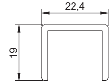
Section No. 30504 0.303 kg/m, per 114.9
