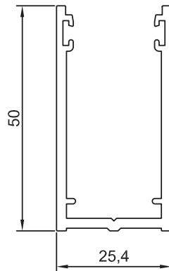
Section No. 33604 0.742 kg/m, per 276
