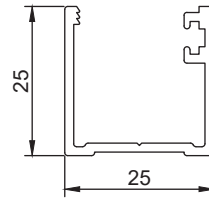
Section No. E770 0.347 kg/m, per 167.7
