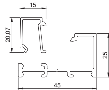
Section No. Z662 0.442 kg/m, per 207.7
