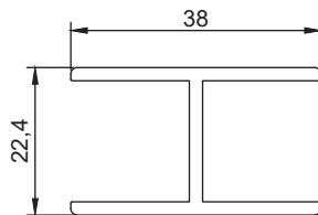
Section No. 30503 0.509 kg/m, per 190.7
