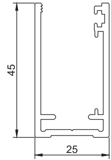
Section No. 31427 0.693 kg/m, per 270.6
