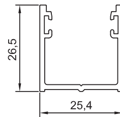
Section No. 33602 0.353 kg/m, per 158.4
