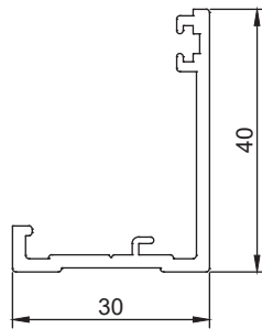
Section No. G675 0.448 kg/m, per 178.2
