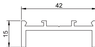
Section No. 5620 0.484 kg/m, per 157.0
