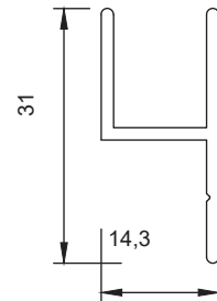
*Section No.J032 0.234 kg/m, per 118
