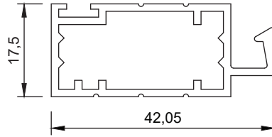
*Section No.218 Flyscreen Door Frame 0.494 kg/m, per 150
