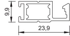
*Section No.219 Flyscreen Window Frame 0.232 kg/m, per 94
