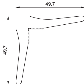
Section No. X429 Stake angle for J058 above 1.475 kg/m, per 193
