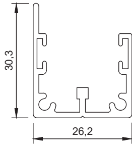
*Section No.30973 Sliding Door Track 0.421 kg/m, per 210
