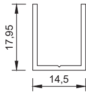
*Section No.X075 0.162 kg/m, per 99
