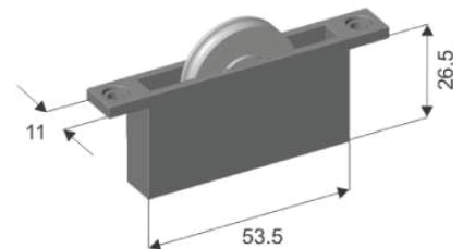
Section No.DR224 Flydoor Carriage Material: Engineere Plastic Standard Roller: DR25 Max Load: 15kg
