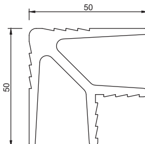
Section No. J688 Stake angle for 9775 above 1.747 kg/m, per 338
