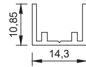
*Section No.X076 0.119 kg/m, per 80
