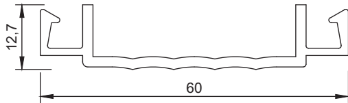
*Section No.J030 0.496 kg/m, per 199
