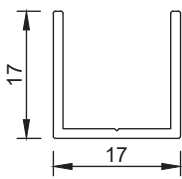
*Section No.31017 0.179 kg/m, per 99
