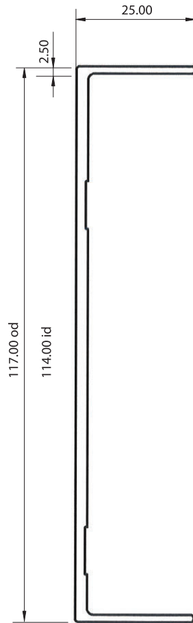
Section No. Z383 / RB-159 114mm Coolroom Channel 0.953 kg/m, per 328
