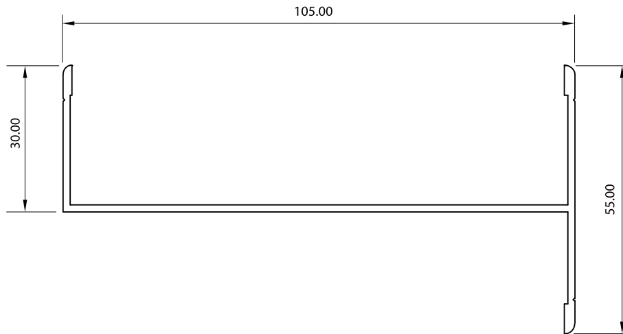
Section No. F3585 100mm Chair Section 0.777kg/m, per 377
