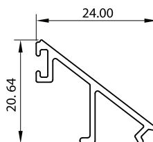
Section No. 36149 Cool Room Single Glazing Bead 0.172 kg/m per 100
