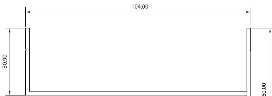
Section No. 36145 100mm Chair Section 0.934 kg/m, per 388
