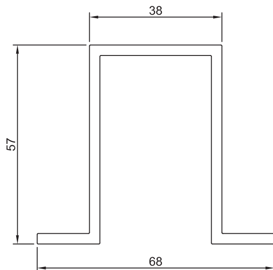
Section No. 38552 1.431 kg/m, per. 356
