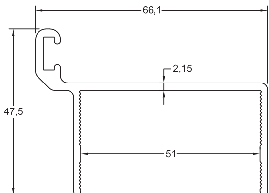
*Section No. 33899 / RB-046 50mm Door Jamb 0.860 kg/m, per. 153
