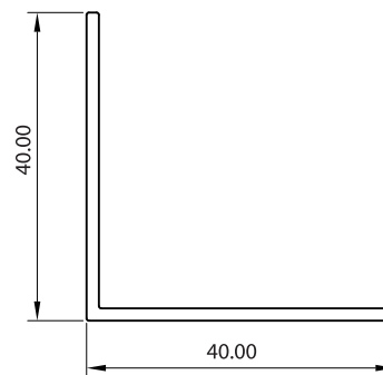
* Section No. RB-129 40mm Angle 0.339 kg/m, per 160
