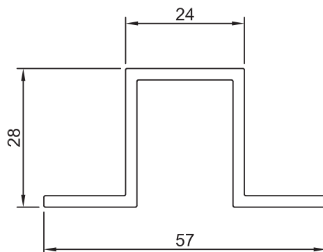
Section No. 38551 0.676 kg/m, per. 220
