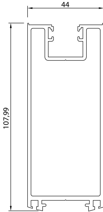
Section No. G611 Wide Lock Stile 1.998 kg/m, Per 421
