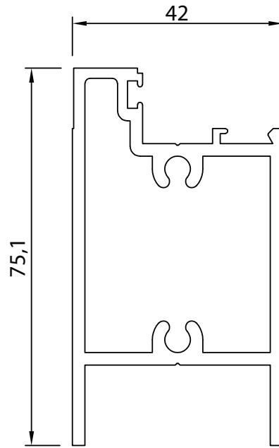
Section No.8163 Top Rail 1.732 kg/m, Per 292
