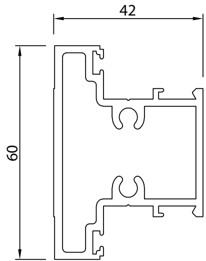
Section No. G251 Narrow Vision Rail 1.400 kg/m, Per 259
