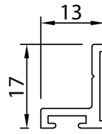
*Section No.6136 Door Stop 0.150 kg/m, Per 72
