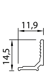
*Section No.31855 Double Glazing Door Bead 0.095 kg/m, Per 53
