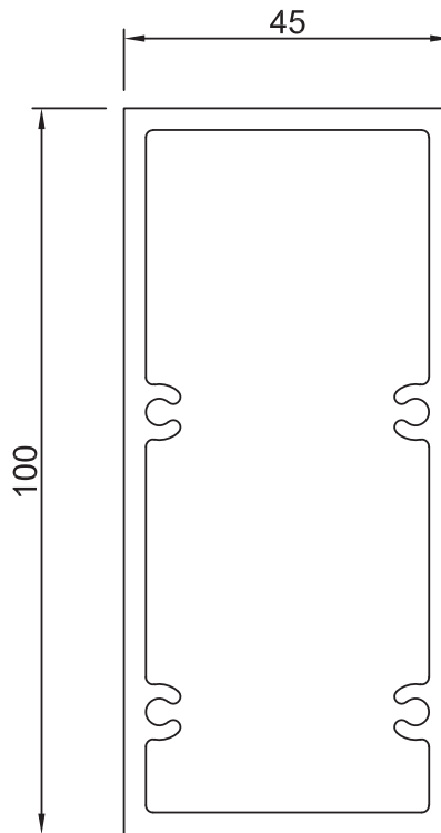
Section No. 9436 Screwports 2.478 kg/m, Per 290
