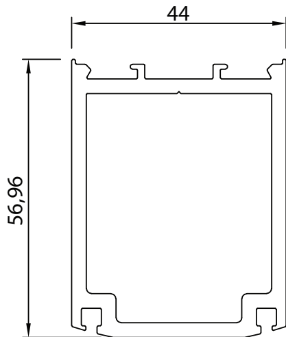
# Section No.33143 Door Stile 1.626 kg/m, Per 248
