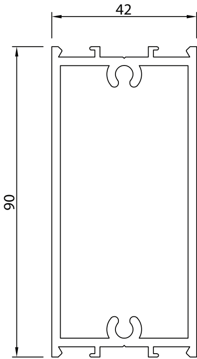
Section No.6100 Beadable Vision Rail 1.961 kg/m, Per 313
