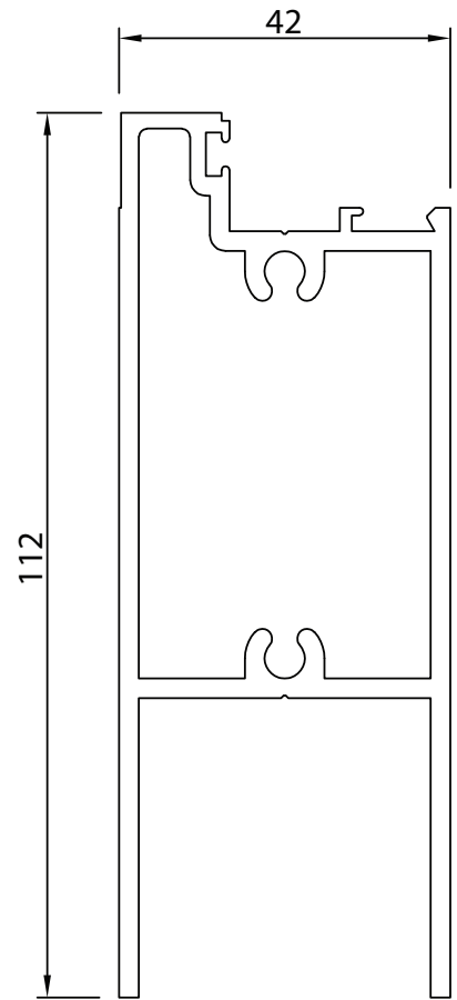
Section No. 8164 Top / Bottom Rail 2.232 kg/m, Per 410
