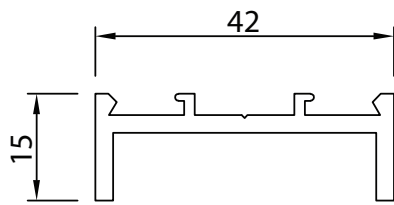
Section No. 5620 Infil Vision Rail 0.484 kg/m, Per 157
