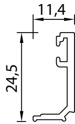
#Section No.32550 Double Glazing Door Bead 0.194 kg/m, Per 87
