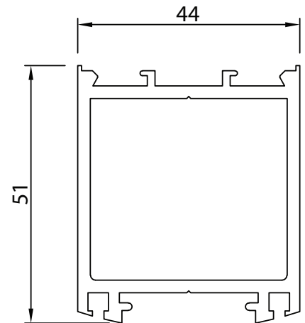
# Section No.31882 Door Rail 2.072 kg/m, Per 384
