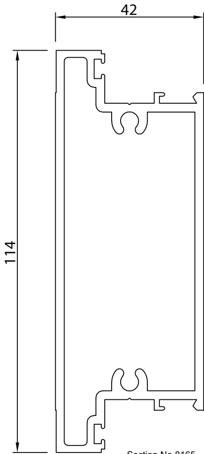
Section No. 8165 Wide Vision Rail 2.285 kg/m, Per 363
