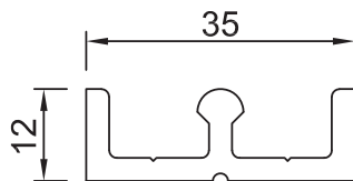
Section No. 6350 Door Track 0.518 kg/m, Per 127
