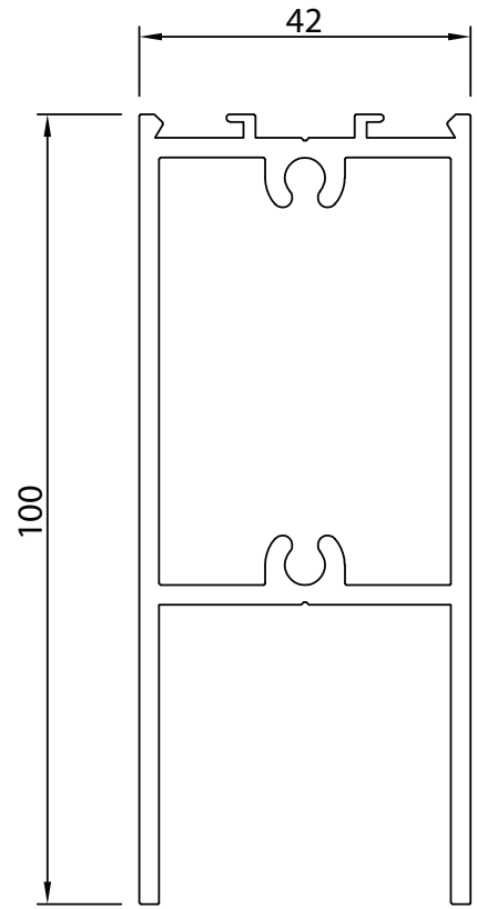
# Section No.31882 Door Rail 2.072 kg/m, Per 384
