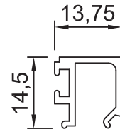
*Section No.5653 Square Bead 0.166 kg/m, Per 98
