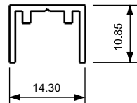
* Section No. X076 Bottom Flyscreen Window Channel 0.138 kg/m per 64
