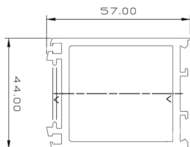
# Section No. 9987 CHC Door Stile 1.617kg/m, per 268.10
