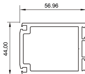
# Section No. 33143 CHC Door Stile 1.626kg/m, per 247.85
